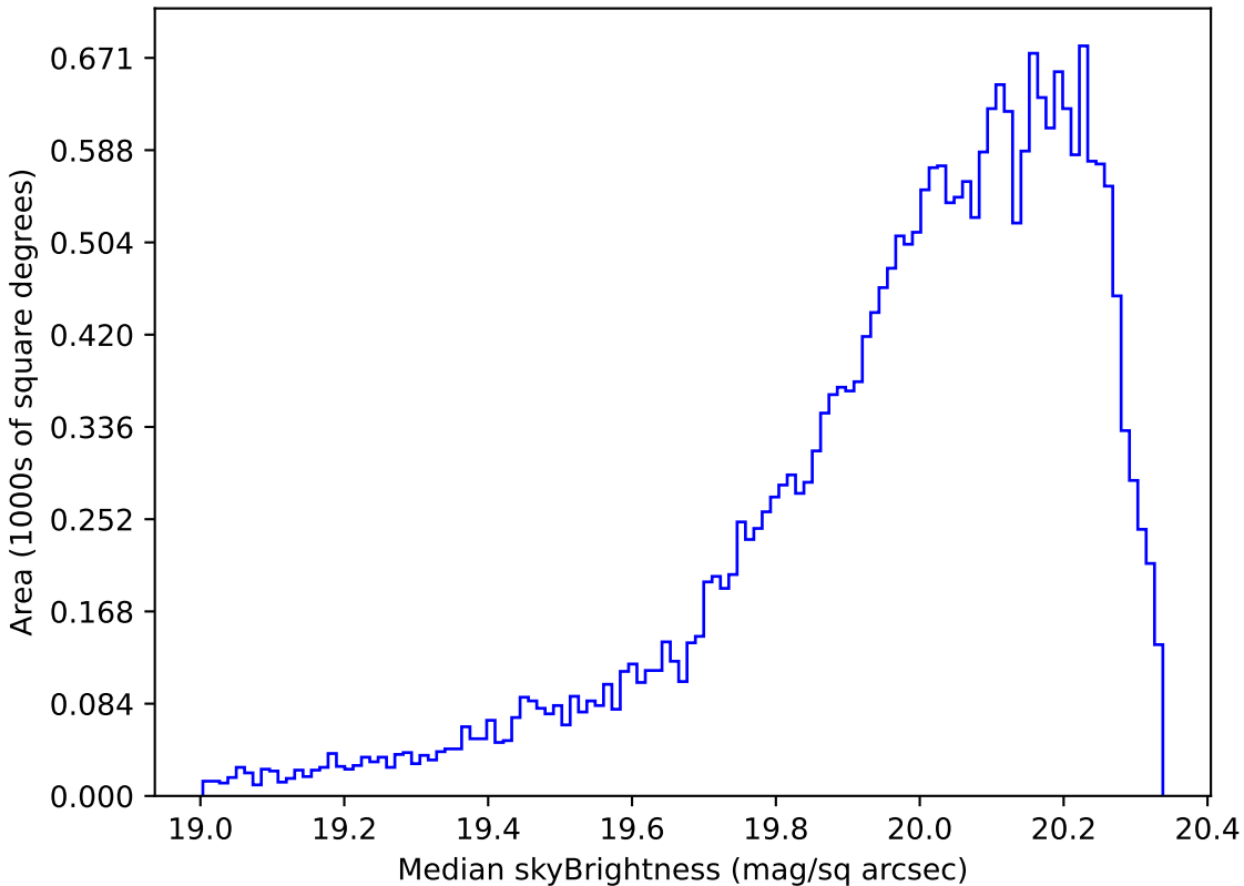
ddf_half_v3.4_10yrs Yr 1 i band: Median skyBrightness
