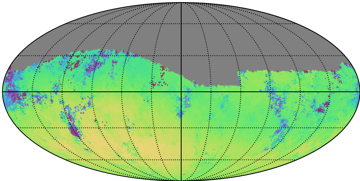
ddf_half_v3.4_10yrs Yr 1 g band: Median skyBrightness
