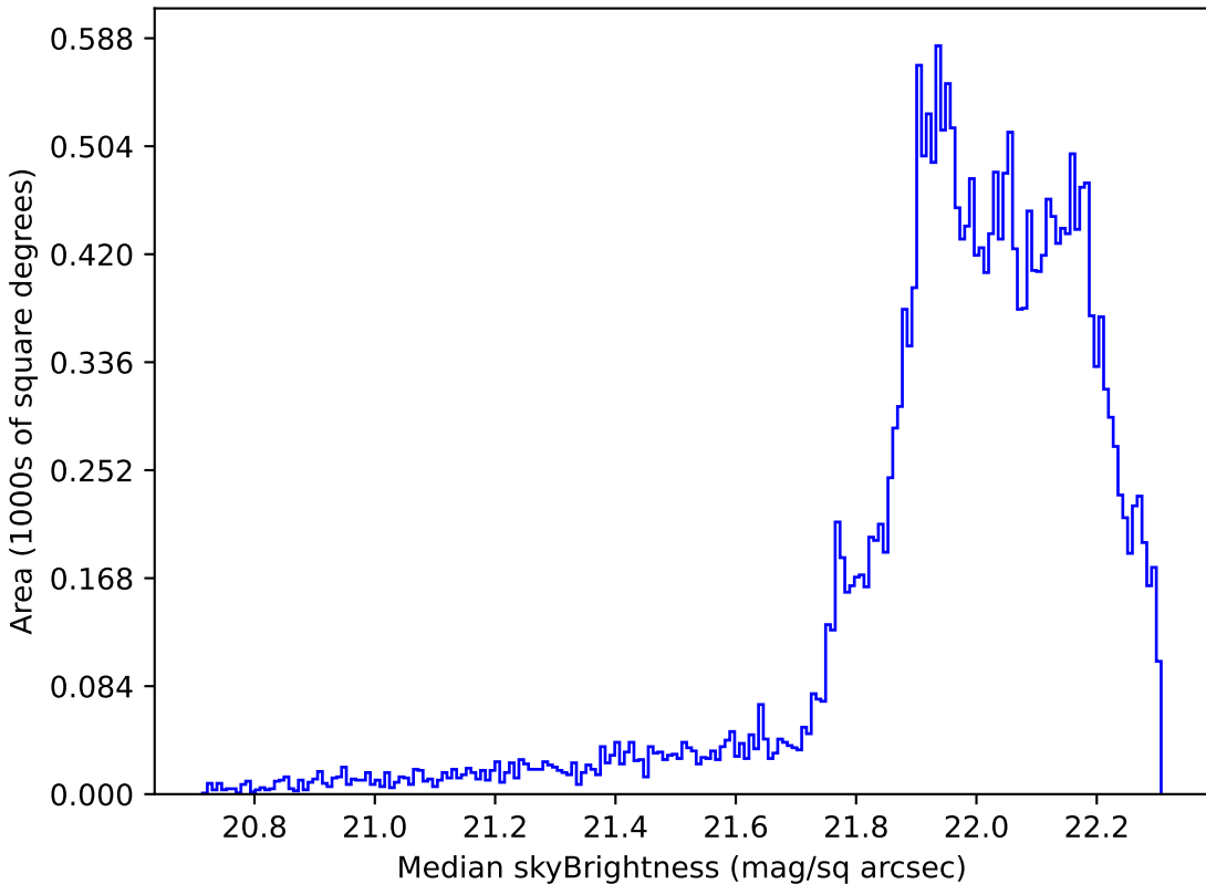
ddf_half_v3.4_10yrs Yr 1 g band: Median skyBrightness
