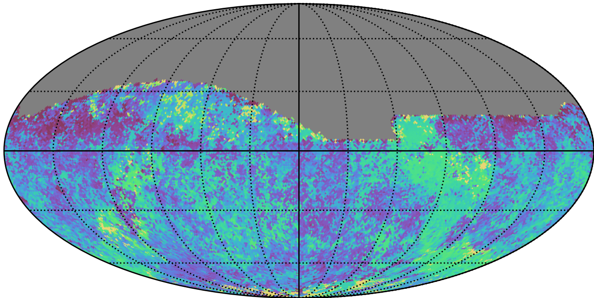
ddf_half_v3.4_10yrs Yr 1 all bands: Median skyBrightness
