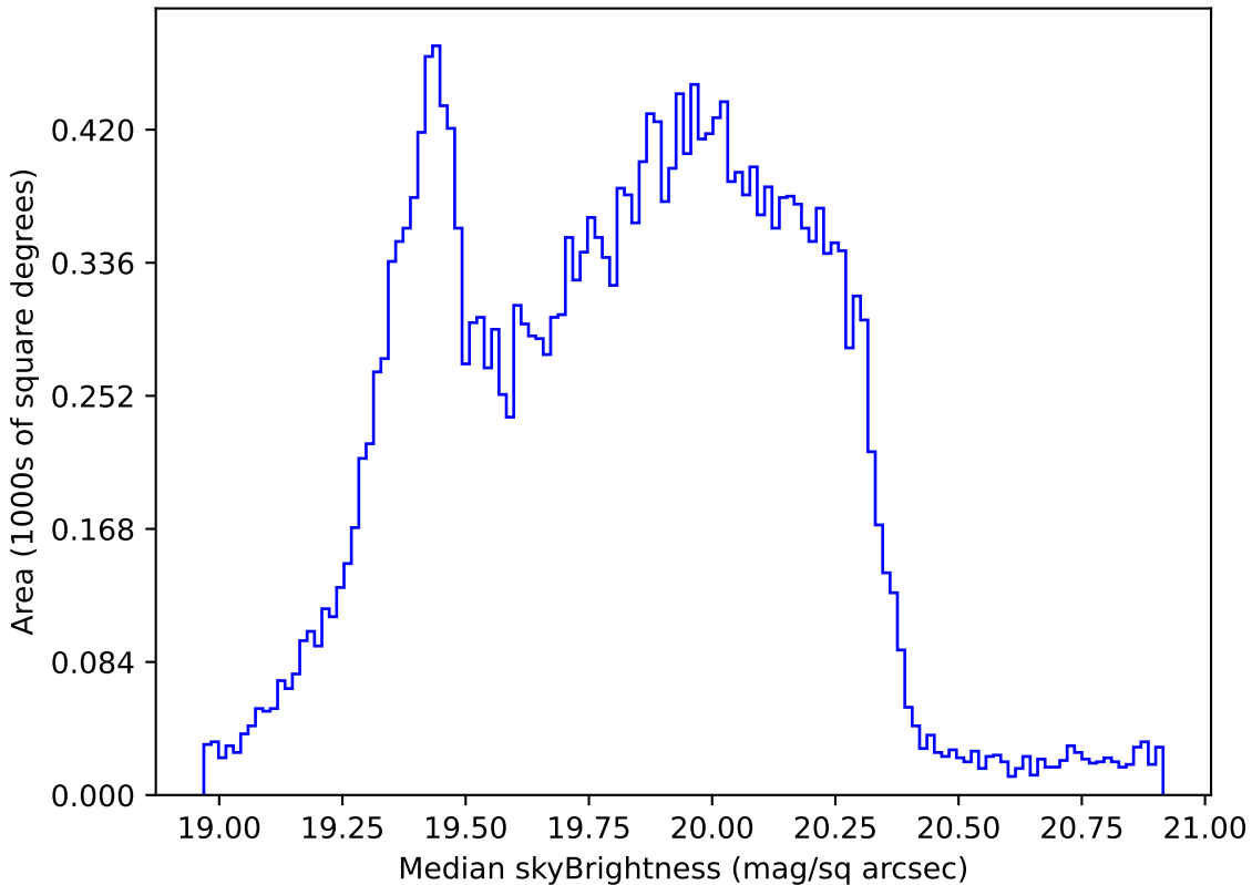
ddf_half_v3.4_10yrs Yr 1 all bands: Median skyBrightness
