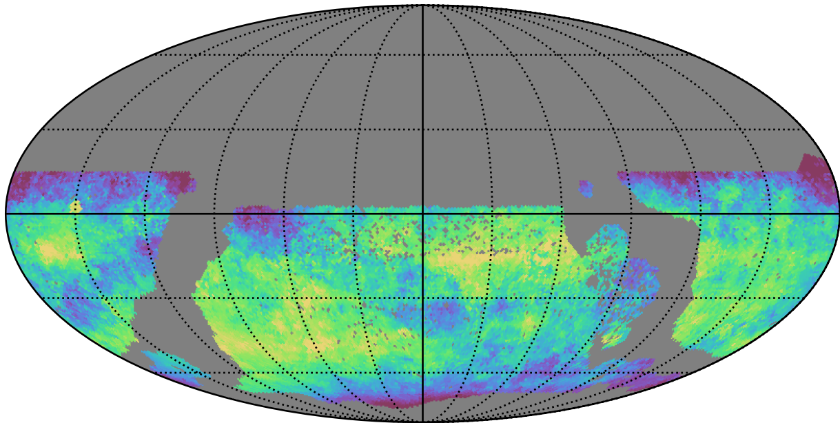
ddf_half_v3.4_10yrs WFD z band: Median skyBrightness
