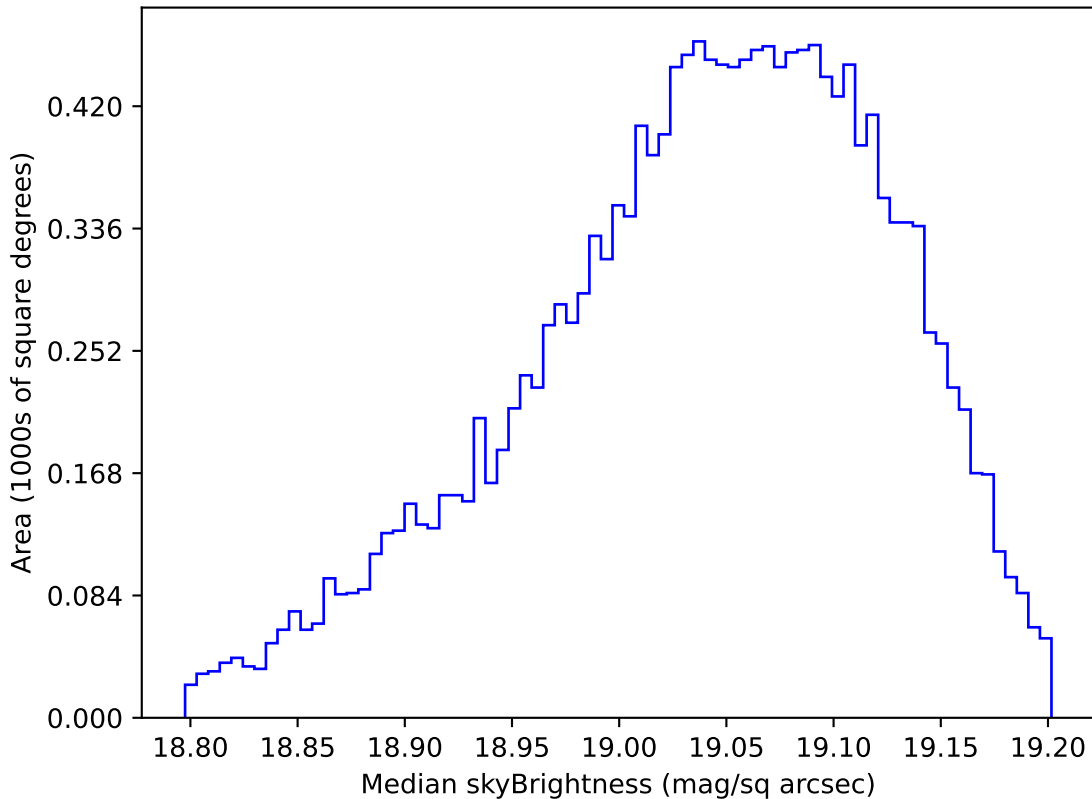
ddf_half_v3.4_10yrs WFD z band: Median skyBrightness
