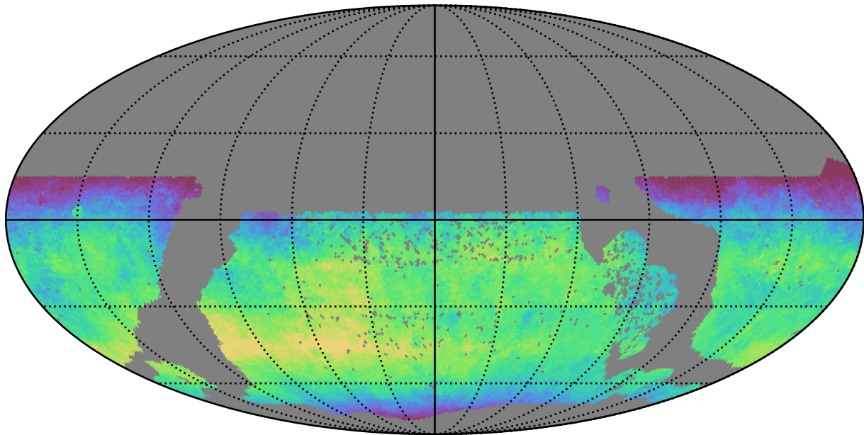
ddf_half_v3.4_10yrs WFD y band: Median skyBrightness
