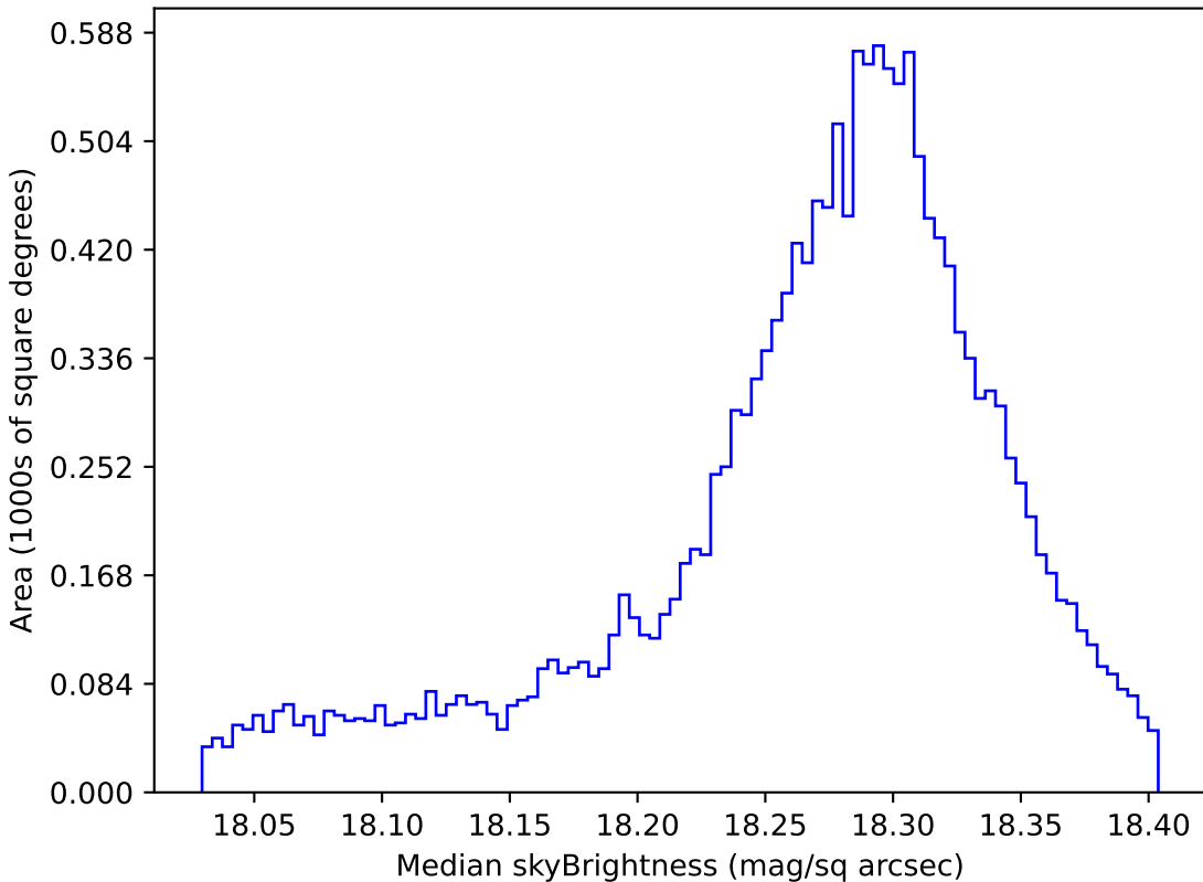
ddf_half_v3.4_10yrs WFD y band: Median skyBrightness
