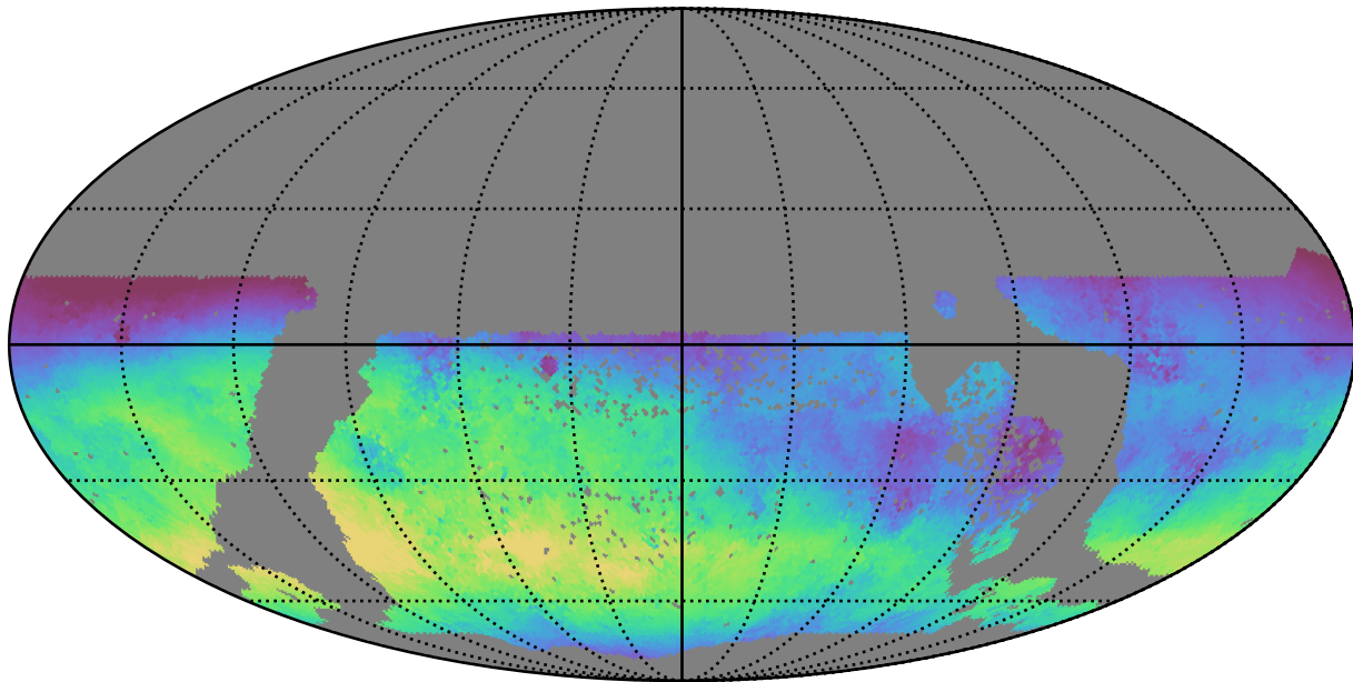
ddf_half_v3.4_10yrs WFD u band: Median skyBrightness
