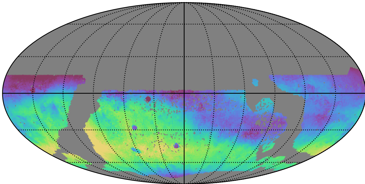
ddf_half_v3.4_10yrs WFD r band: Median skyBrightness
