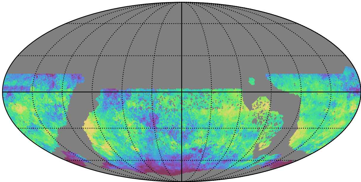
ddf_half_v3.4_10yrs WFD i band: Median skyBrightness
