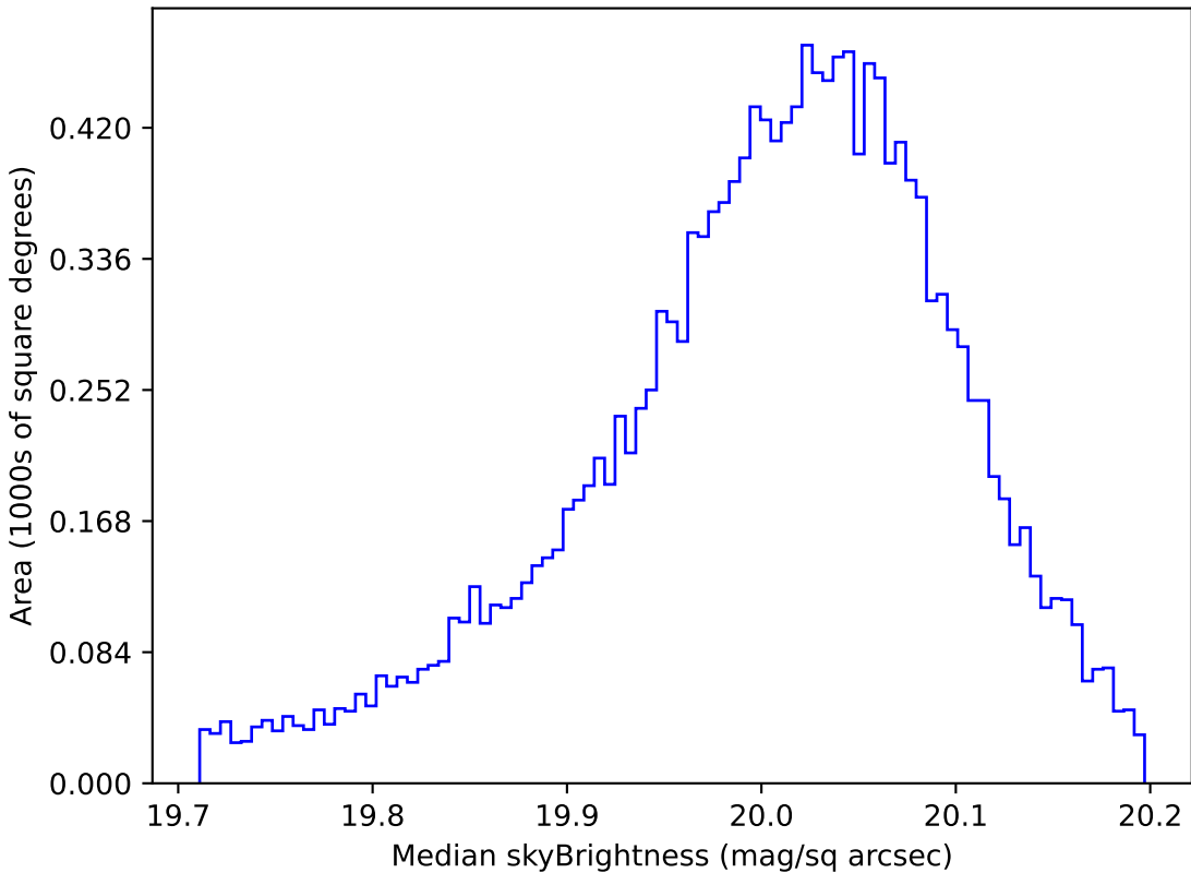
ddf_half_v3.4_10yrs WFD i band: Median skyBrightness
