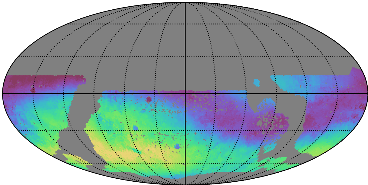
ddf_half_v3.4_10yrs WFD g band: Median skyBrightness
