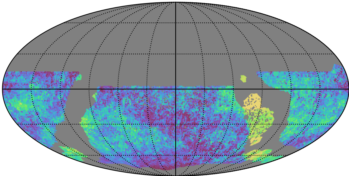
ddf_half_v3.4_10yrs WFD all bands: Median skyBrightness
