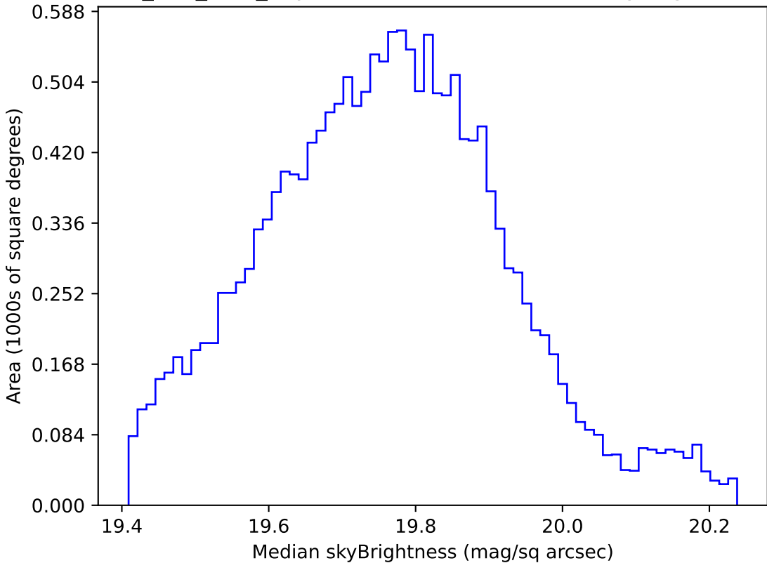
ddf_half_v3.4_10yrs WFD all bands: Median skyBrightness
