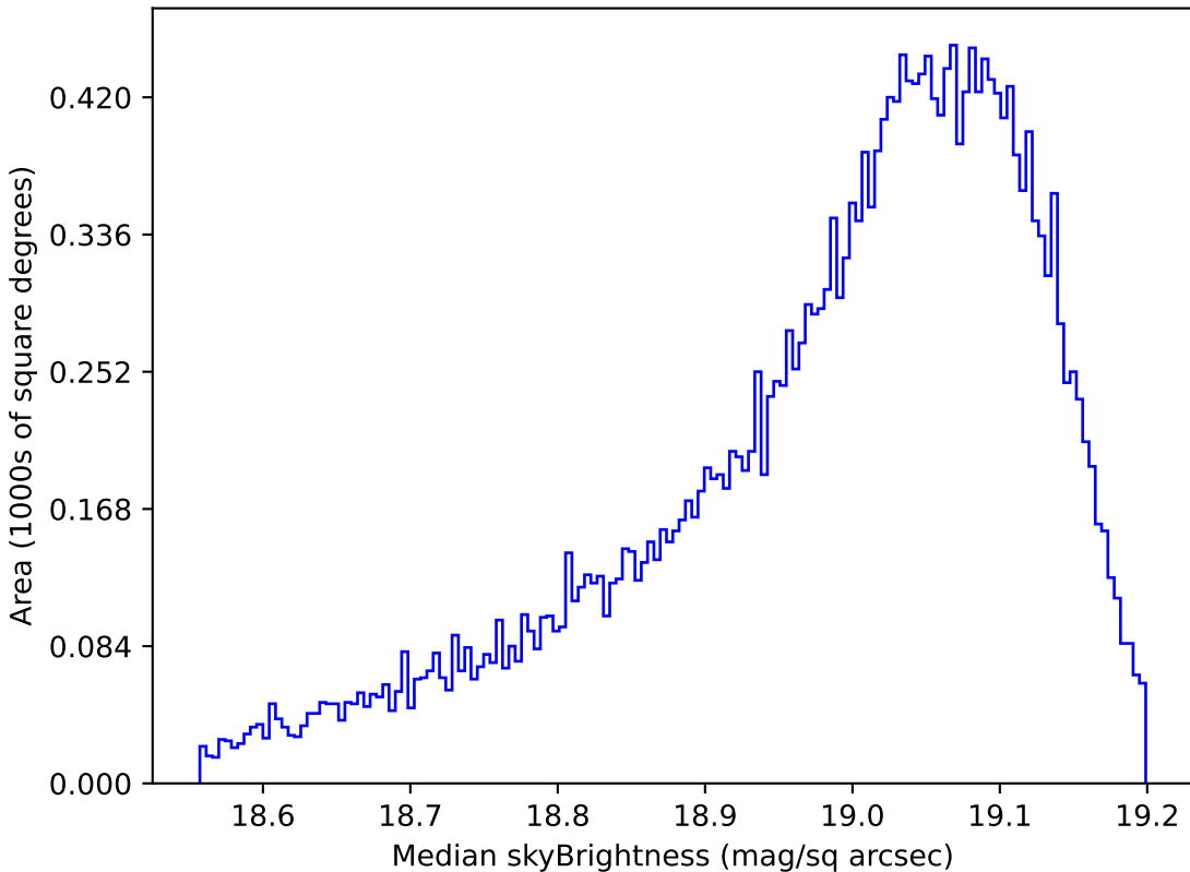
ddf_half_v3.4_10yrs All sky z band: Median skyBrightness
