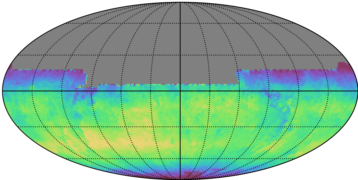
ddf_half_v3.4_10yrs All sky y band: Median skyBrightness
