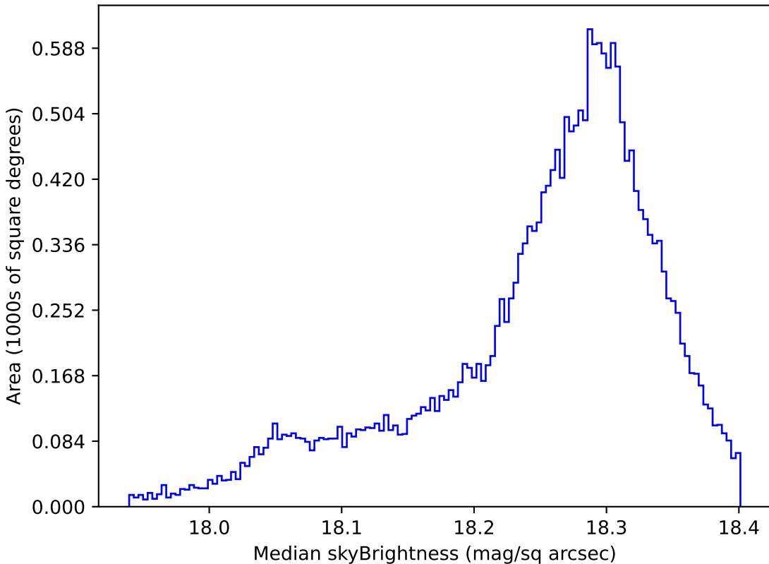
ddf_half_v3.4_10yrs All sky y band: Median skyBrightness
