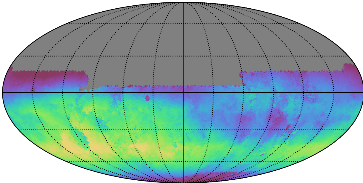
ddf_half_v3.4_10yrs All sky u band: Median skyBrightness
