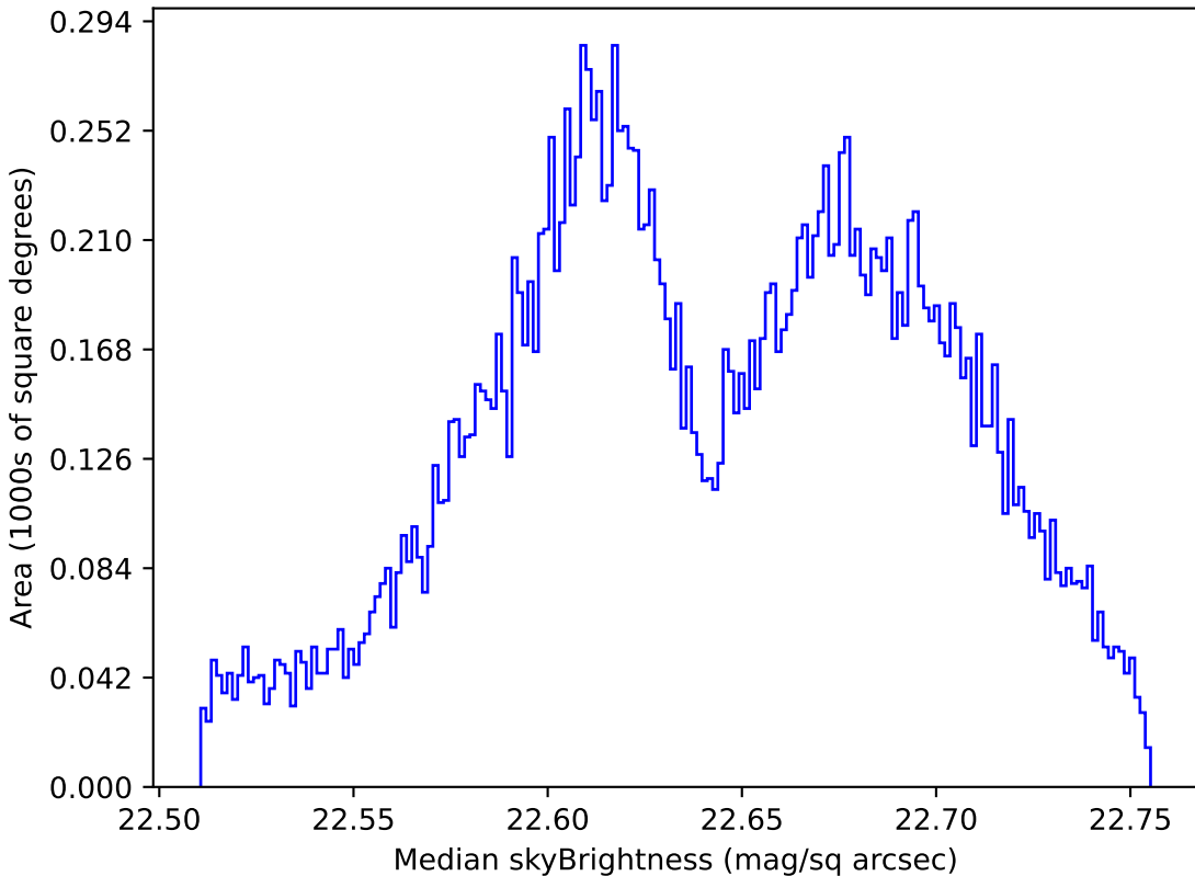
ddf_half_v3.4_10yrs All sky u band: Median skyBrightness
