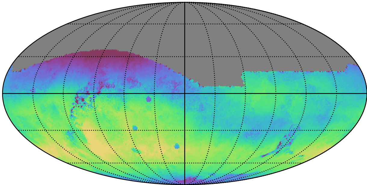
ddf_half_v3.4_10yrs All sky r band: Median skyBrightness
