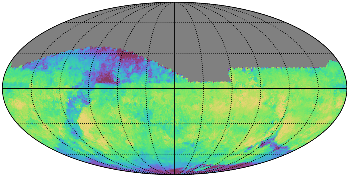
ddf_half_v3.4_10yrs All sky i band: Median skyBrightness
