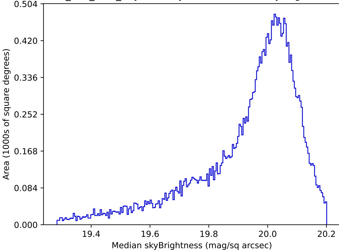
ddf_half_v3.4_10yrs All sky i band: Median skyBrightness
