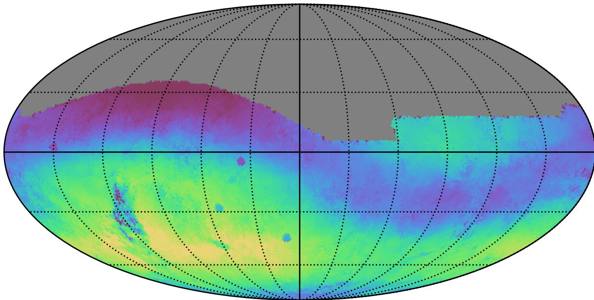
ddf_half_v3.4_10yrs All sky g band: Median skyBrightness
