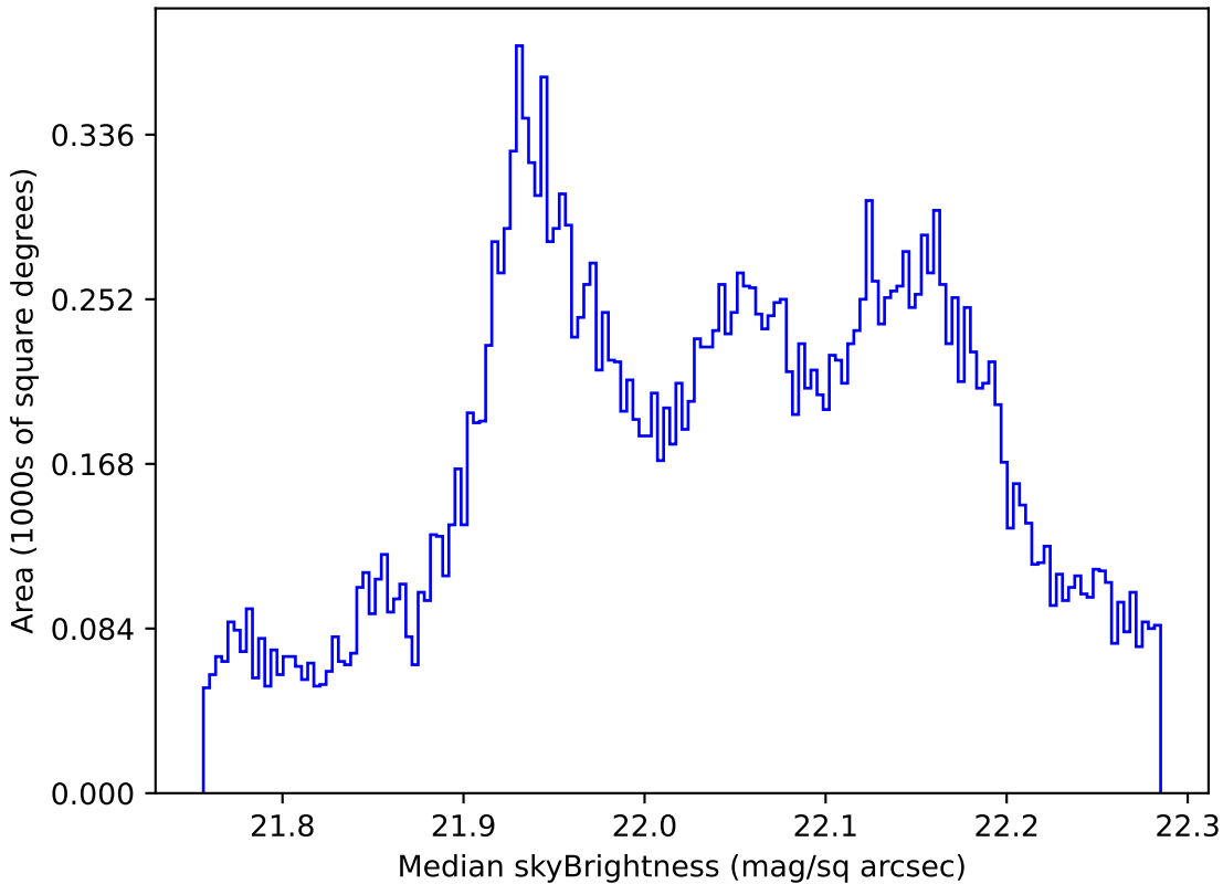
ddf_half_v3.4_10yrs All sky g band: Median skyBrightness
