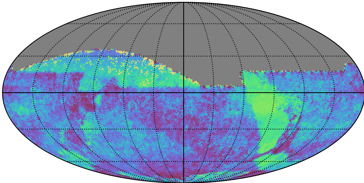
ddf_half_v3.4_10yrs All sky all bands: Median skyBrightness
