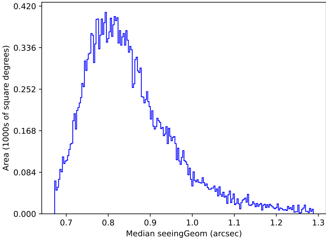
ddf_half_v3.4_10yrs Yr 1 z band: Median seeingGeom
