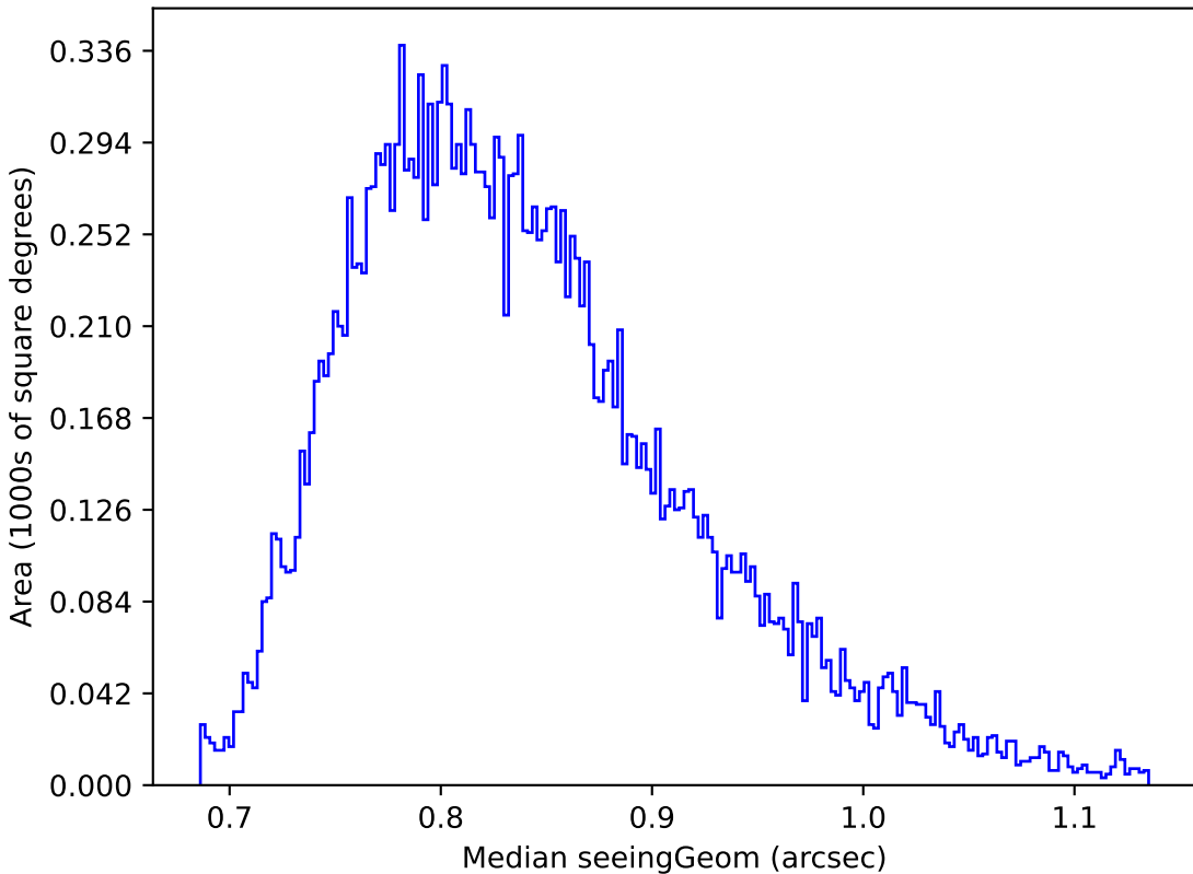
ddf_half_v3.4_10yrs Yr 1 y band: Median seeingGeom
