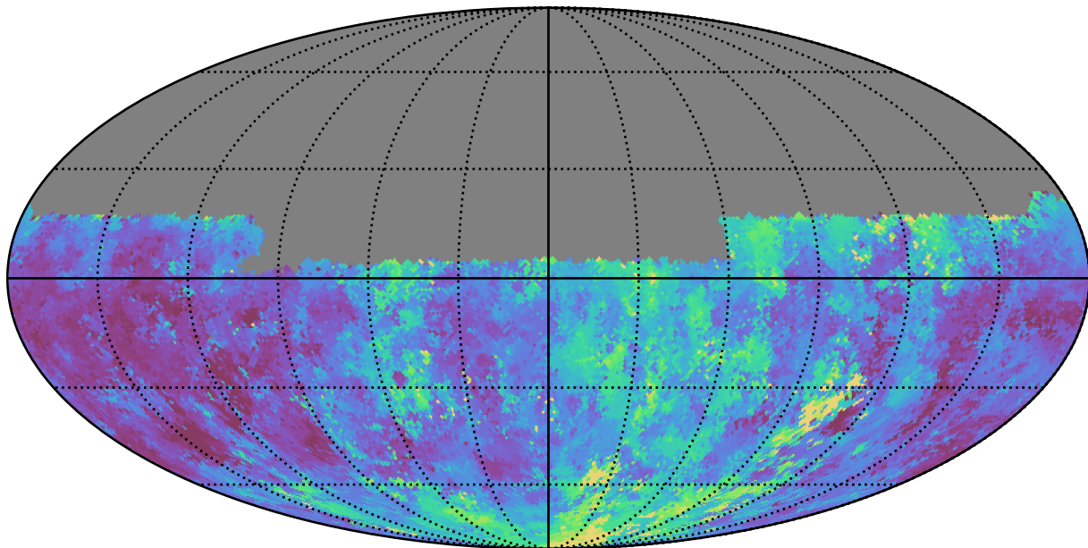
ddf_half_v3.4_10yrs Yr 1 u band: Median seeingGeom
