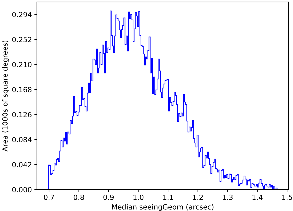
ddf_half_v3.4_10yrs Yr 1 u band: Median seeingGeom
