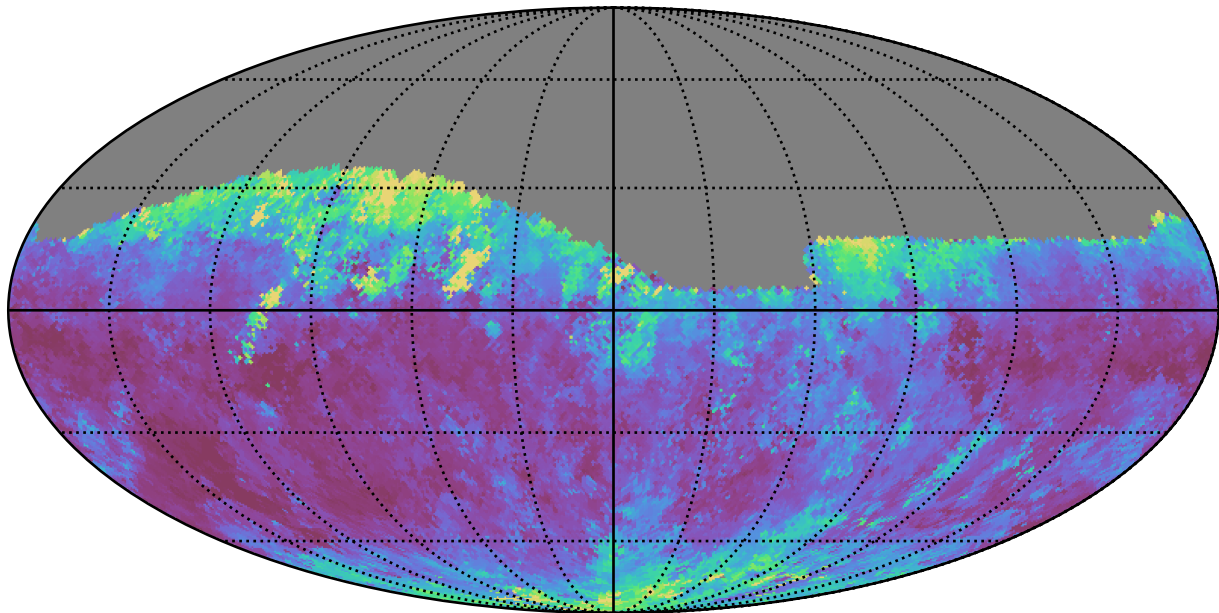
ddf_half_v3.4_10yrs Yr 1 r band: Median seeingGeom
