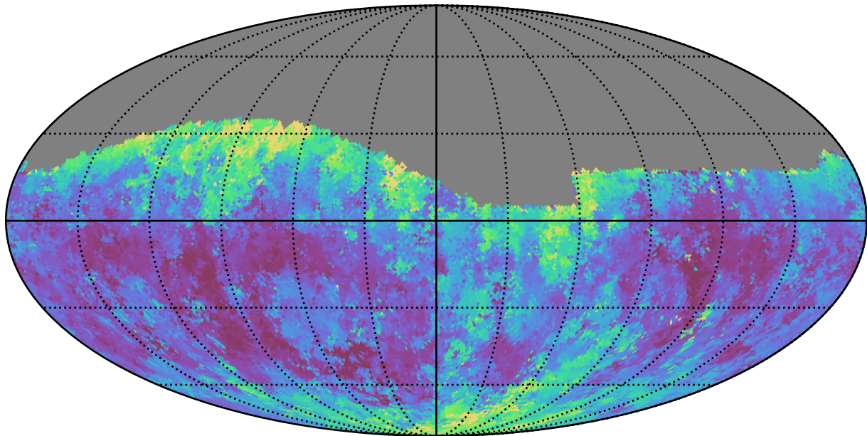
ddf_half_v3.4_10yrs Yr 1 g band: Median seeingGeom
