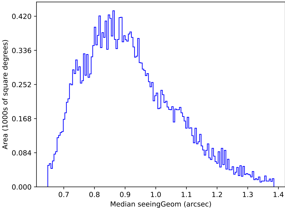
ddf_half_v3.4_10yrs Yr 1 g band: Median seeingGeom
