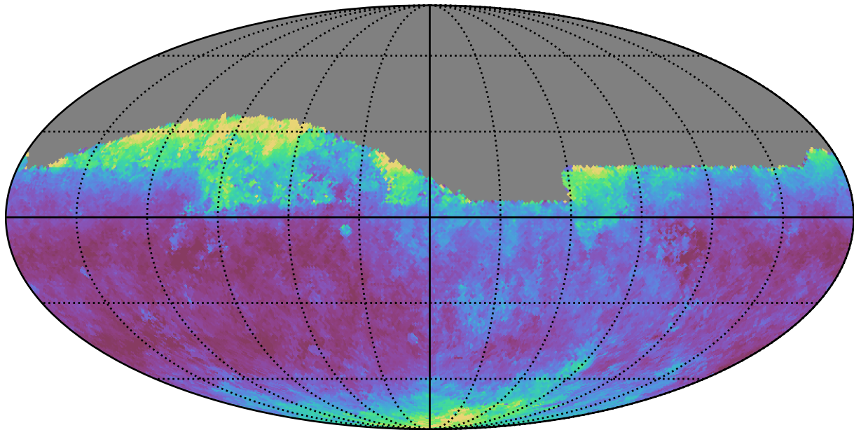
ddf_half_v3.4_10yrs Yr 1 all bands: Median seeingGeom
