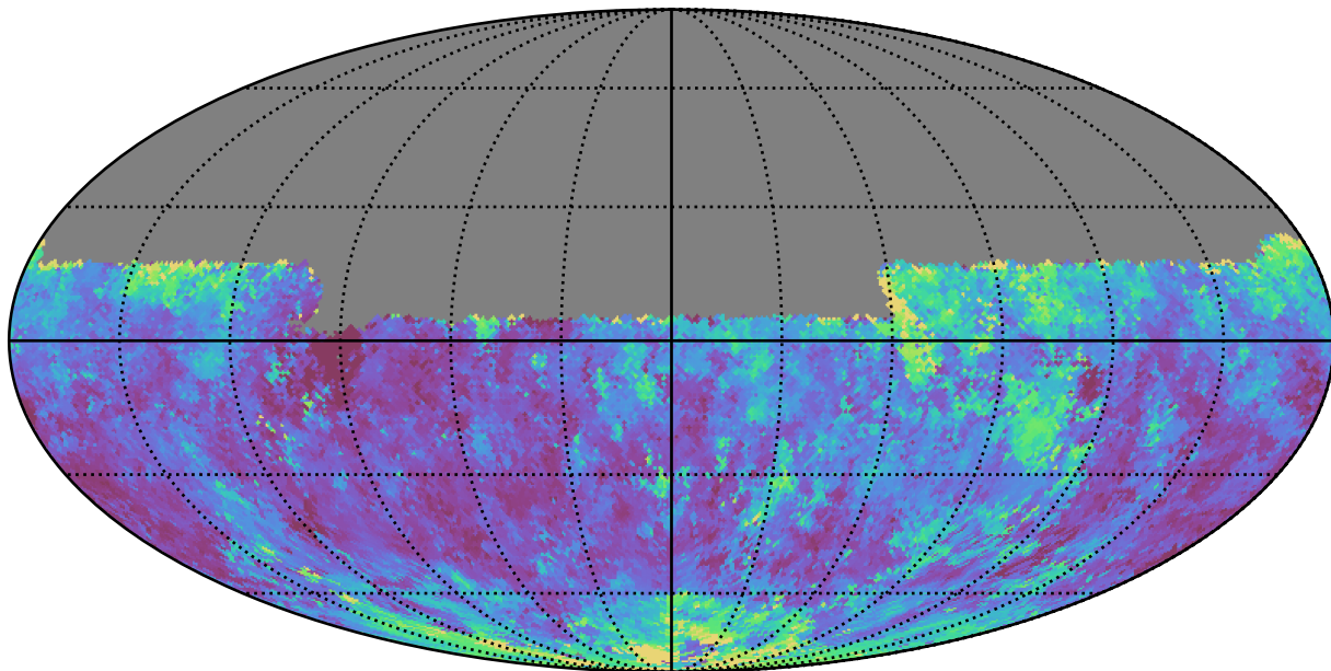
ddf_half_v3.4_10yrs Yr 1 y band: Median seeingEff
