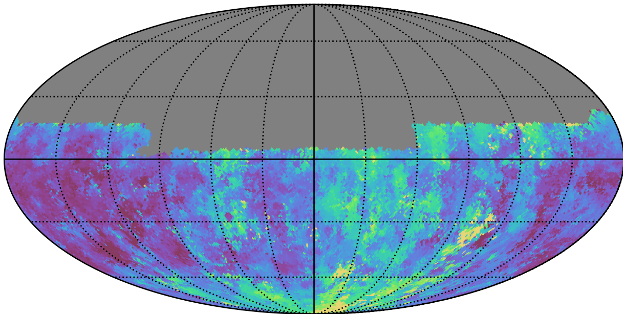
ddf_half_v3.4_10yrs Yr 1 u band: Median seeingEff
