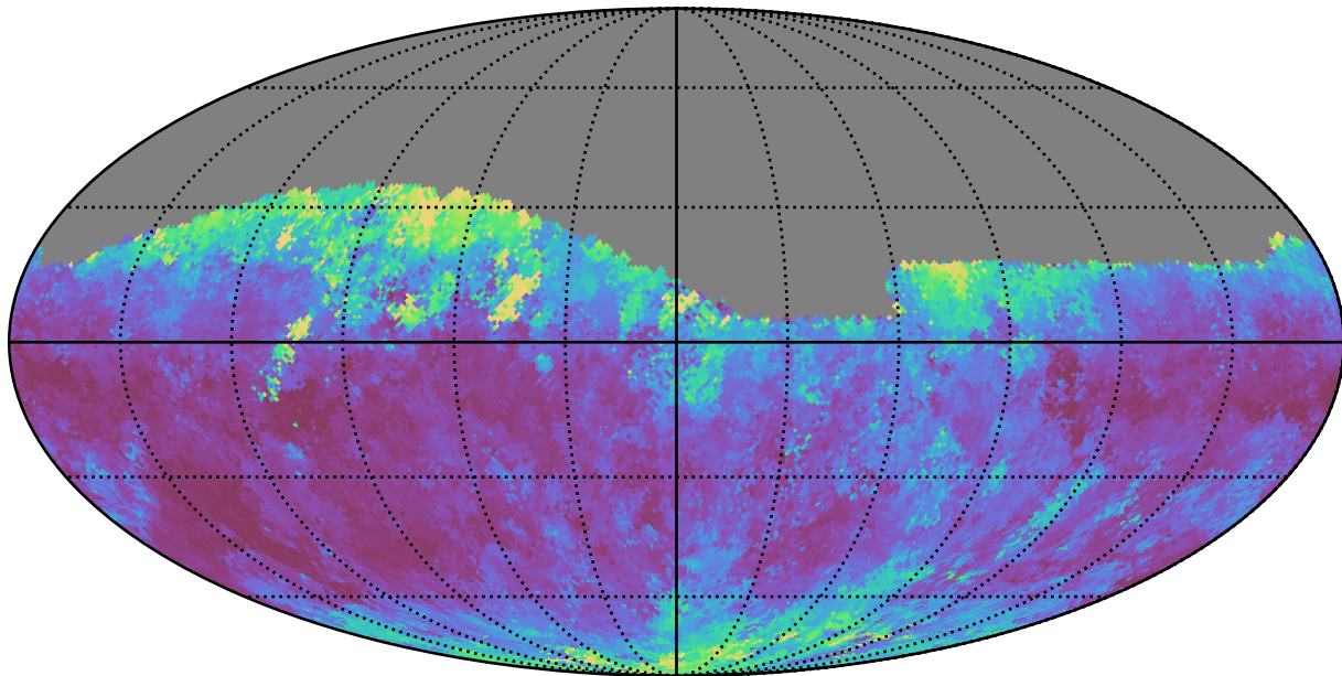
ddf_half_v3.4_10yrs Yr 1 r band: Median seeingEff
