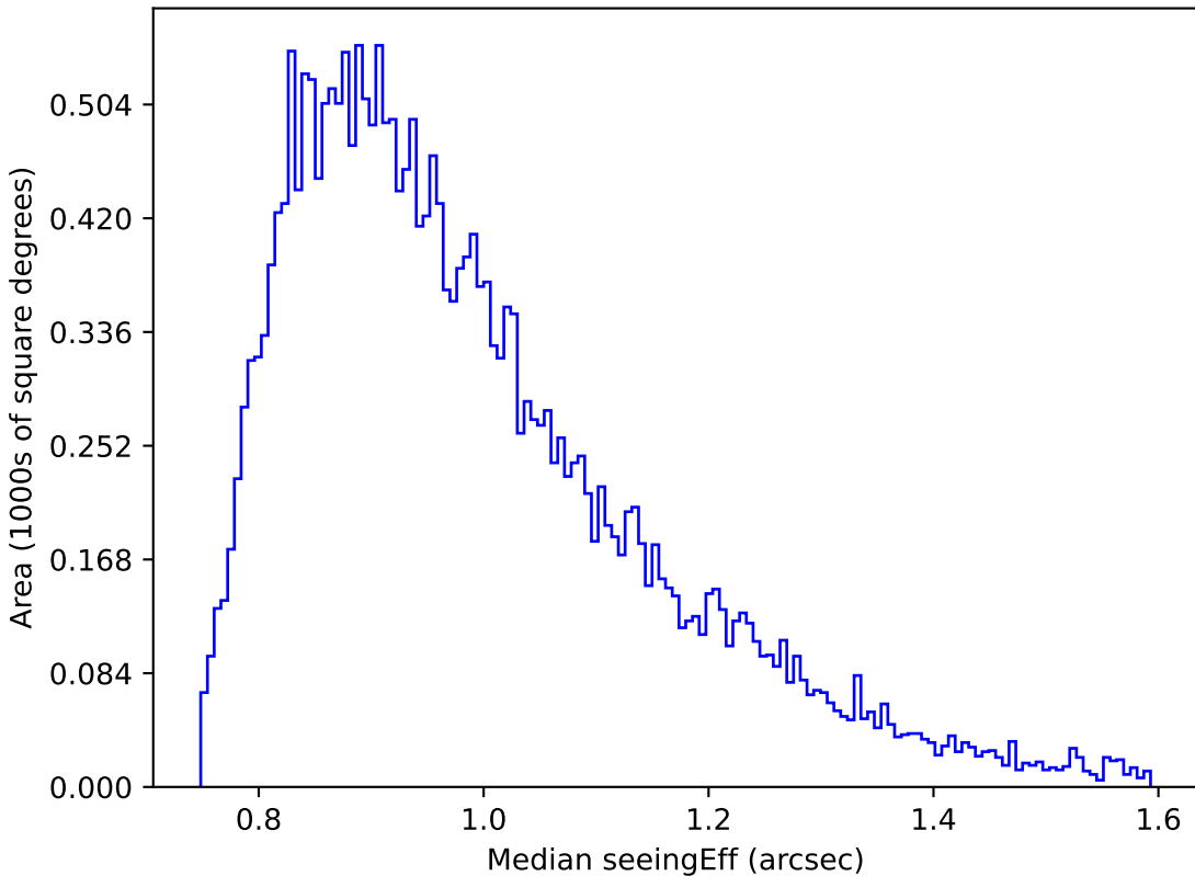
ddf_half_v3.4_10yrs Yr 1 r band: Median seeingEff
