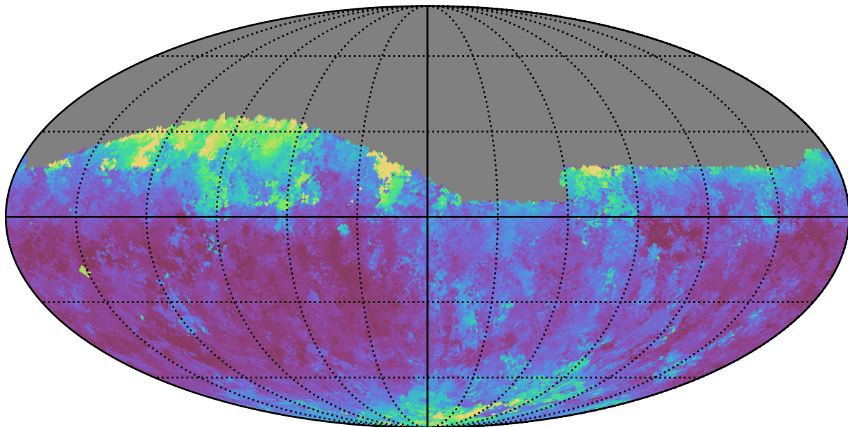
ddf_half_v3.4_10yrs Yr 1 i band: Median seeingEff
