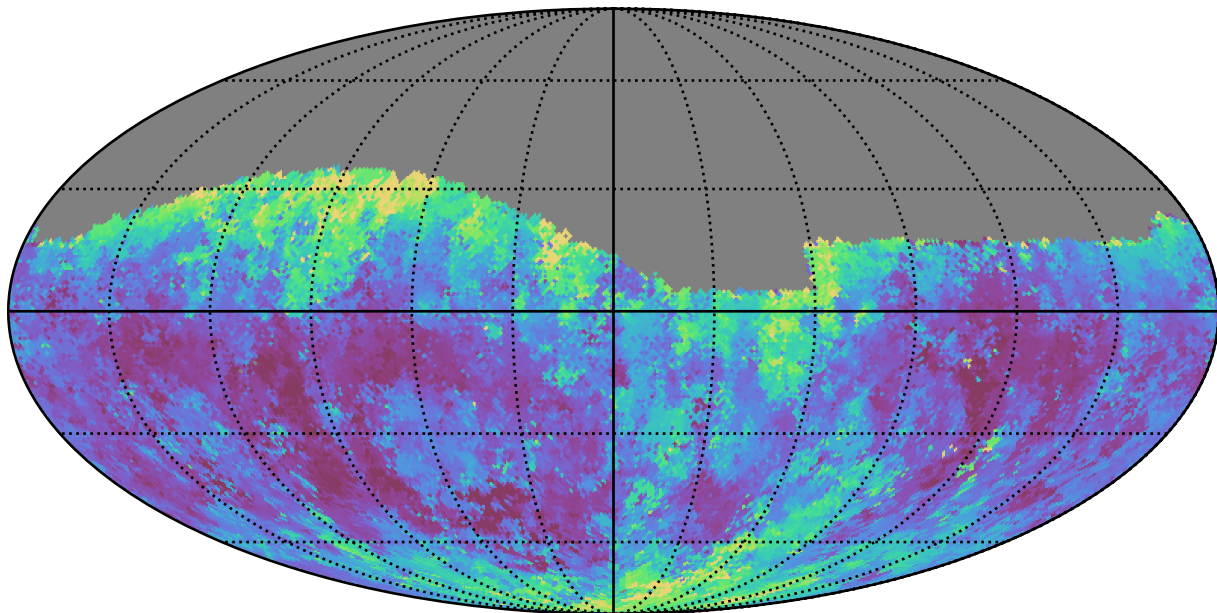
ddf_half_v3.4_10yrs Yr 1 g band: Median seeingEff
