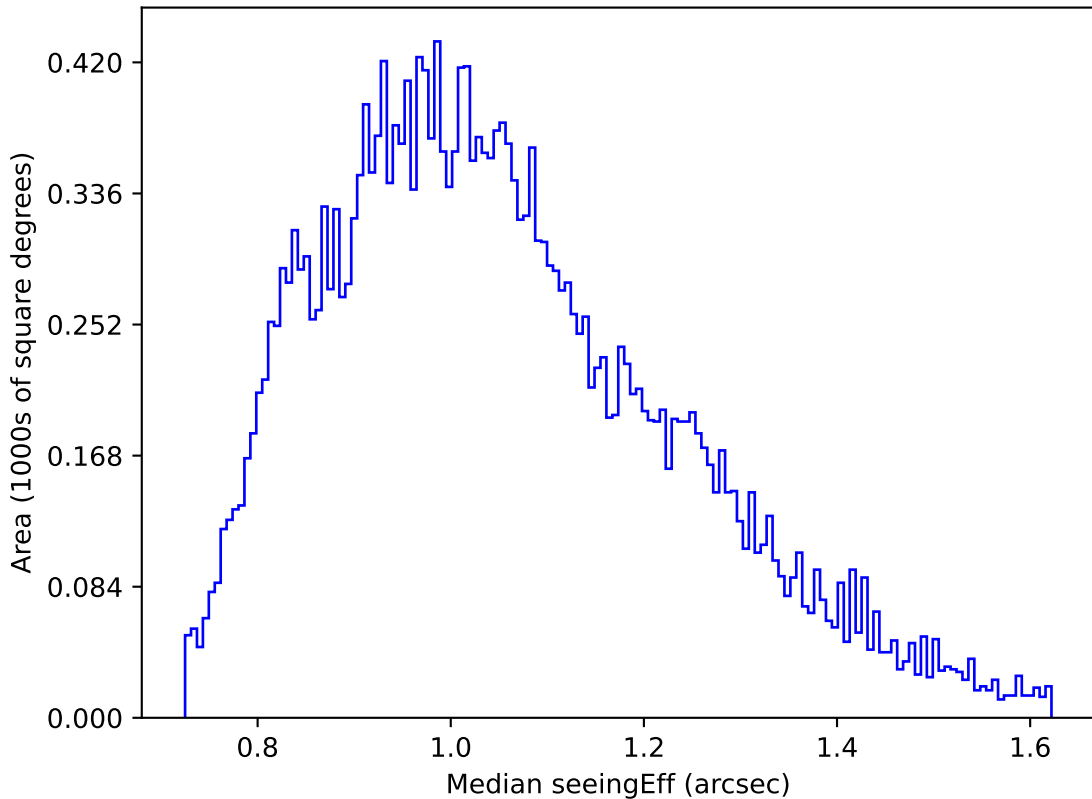
ddf_half_v3.4_10yrs Yr 1 g band: Median seeingEff
