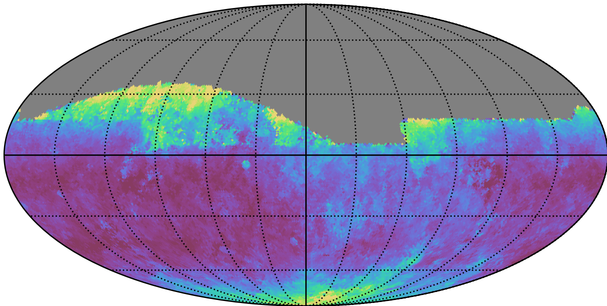
ddf_half_v3.4_10yrs Yr 1 all bands: Median seeingEff
