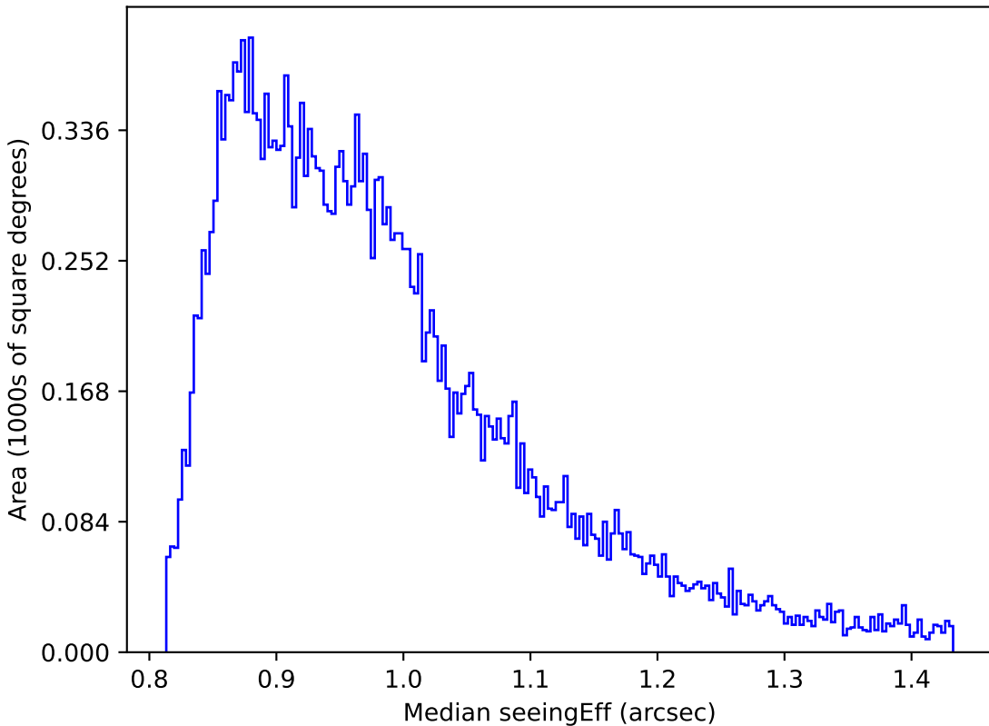
ddf_half_v3.4_10yrs Yr 1 all bands: Median seeingEff
