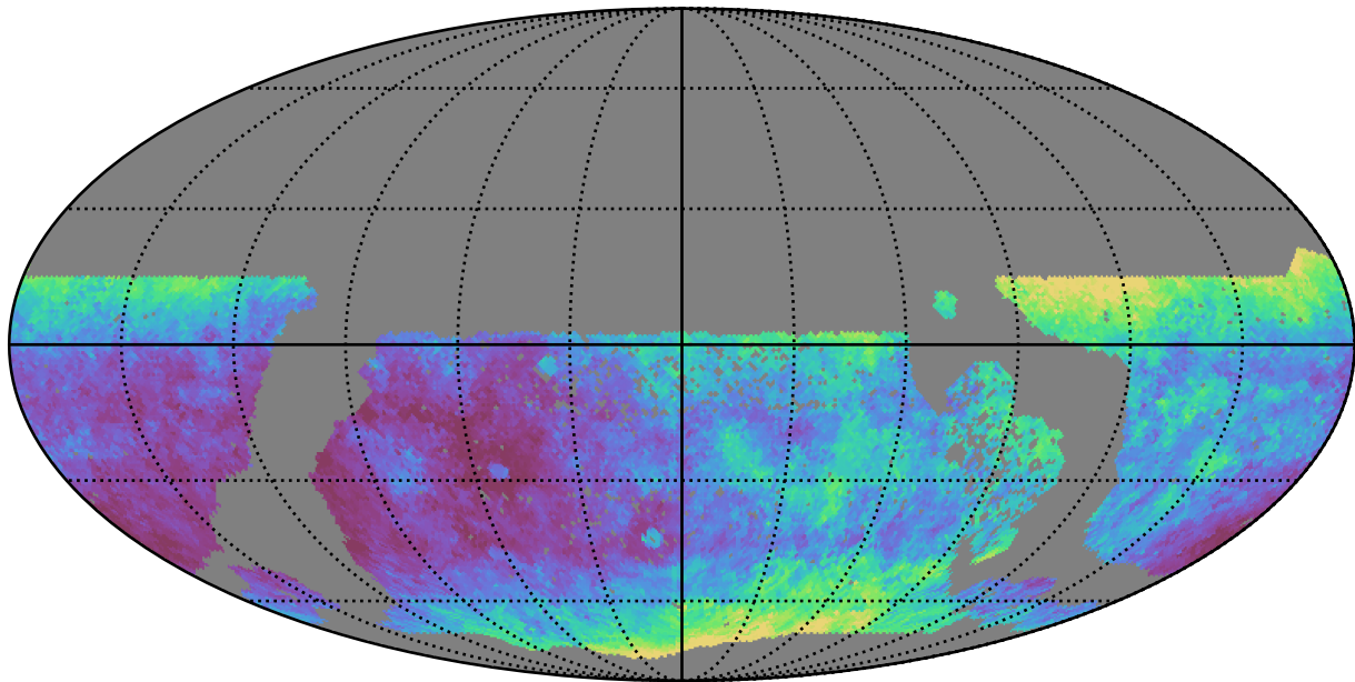
ddf_half_v3.4_10yrs WFD y band: Median seeingEff
