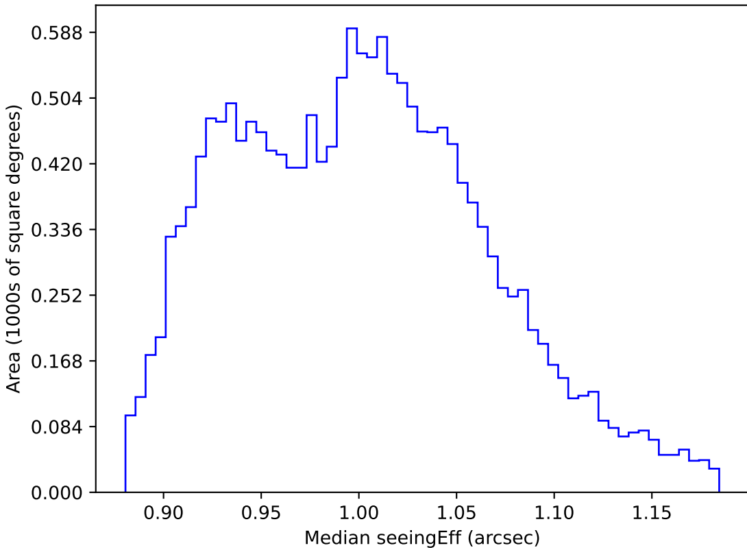
ddf_half_v3.4_10yrs WFD y band: Median seeingEff
