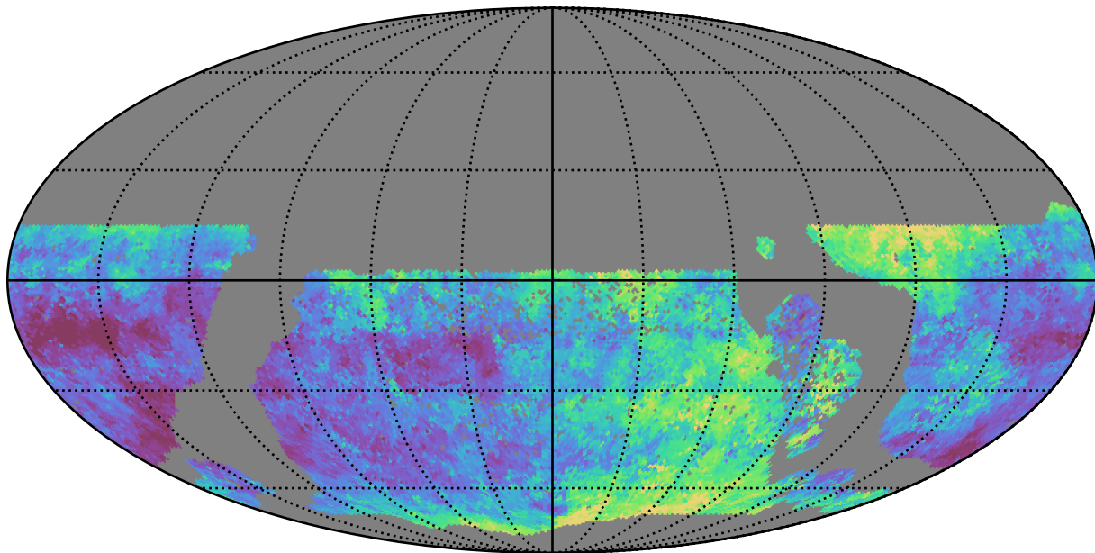
ddf_half_v3.4_10yrs WFD u band: Median seeingEff
