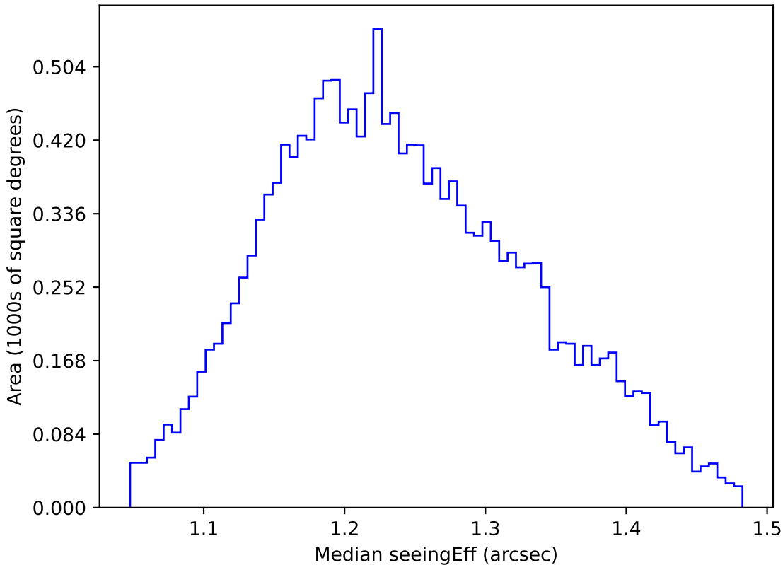
ddf_half_v3.4_10yrs WFD u band: Median seeingEff
