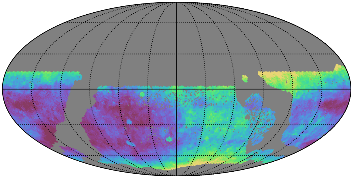
ddf_half_v3.4_10yrs WFD r band: Median seeingEff
