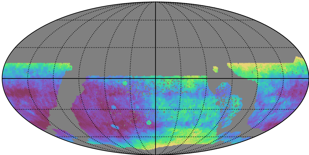
ddf_half_v3.4_10yrs WFD i band: Median seeingEff
